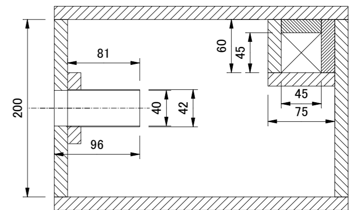
Section "EE"
