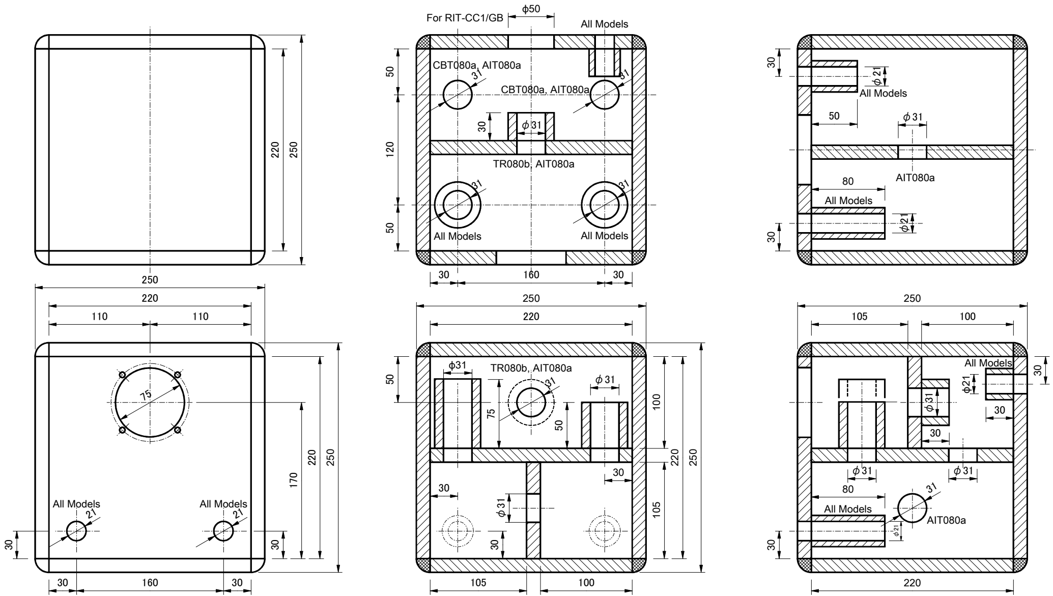
TR080b / AIT080a / CBT080a Assembly (Actual Drawing)
