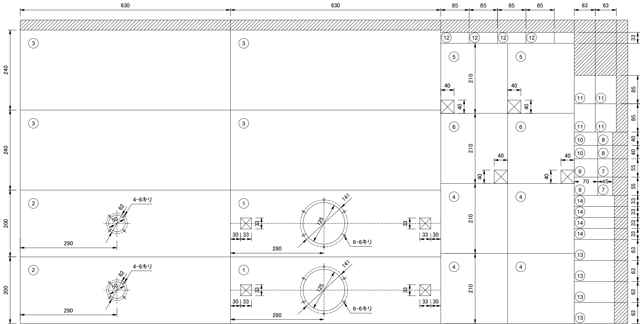
DU130a cutting plan
